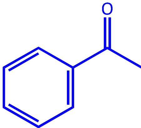
Acetophenone
