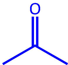
Acetone
