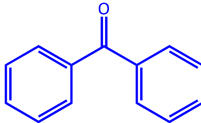
Benzophenone
