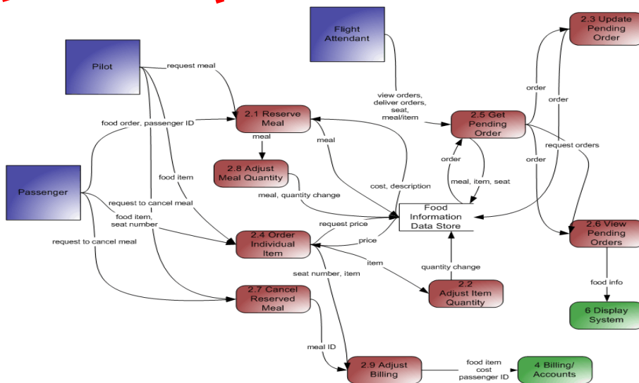
2.3: Data Requirement (ER Diagram)
