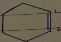
cyclohexene
