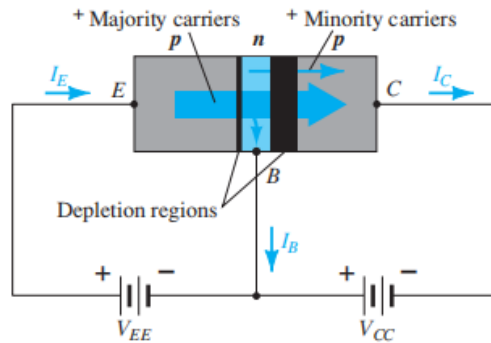
Figure 5.0 Majority and minority carrier flow of a pnp transistor
