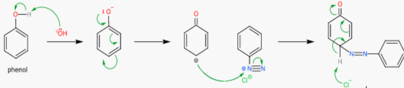
Mechanism of synthesis of Phenyl orange dye
